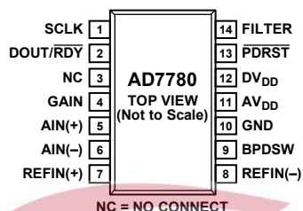
Figure 6. SOIC Pin Configuration
